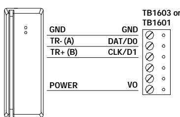
Typical 2-wire RS-485 Device (such as OSDP Reader)
