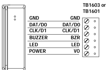
Typical D1/D0 or Clock/Data Reader
